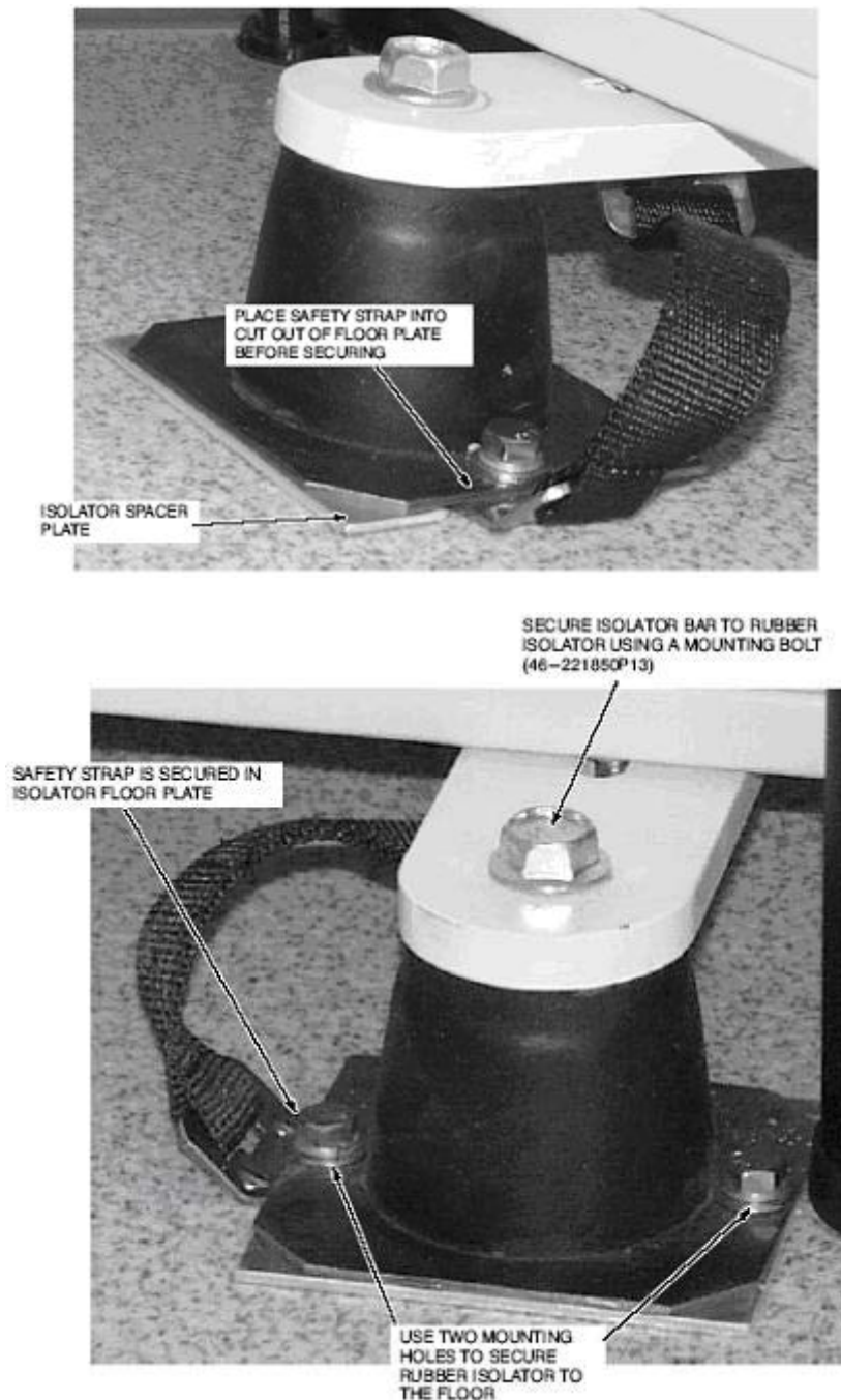
Illustration 8: Safety strap Alignment Details
