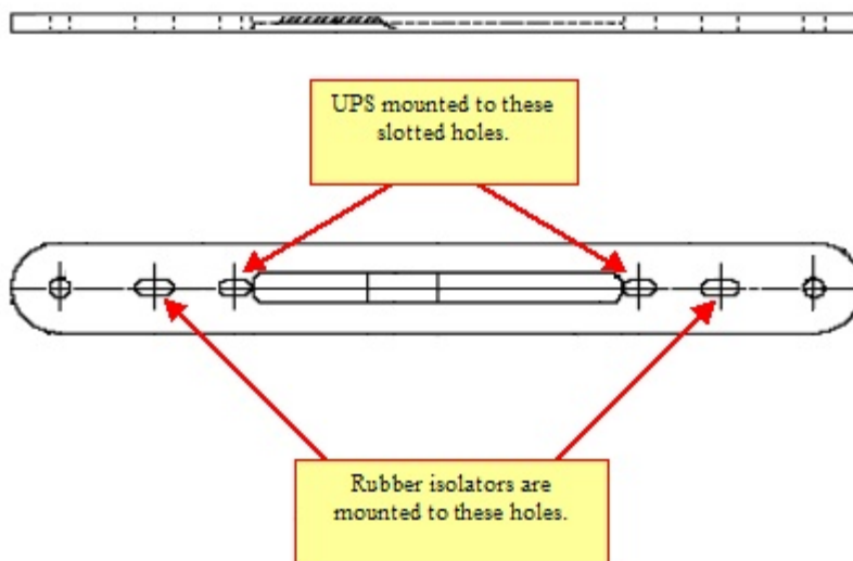
Illustration 4: Isolator Bars (5169868)
