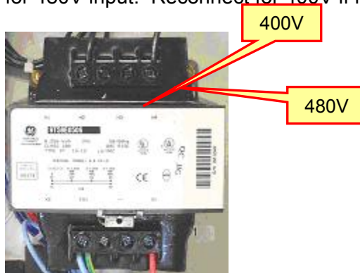
Illustration 13: A1 Panel Control Transformer
