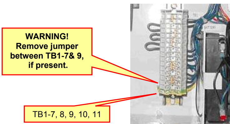
Illustration 12: A1 Panel TB1 Terminals
